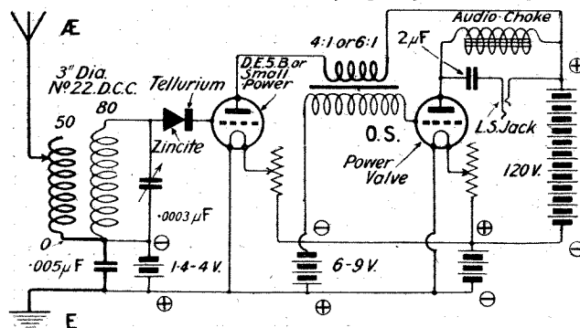
Fig. 1.—The circuit of the set described. It is important that the crystals of the detector be placed in the positions shown here, the zincite being nearest to the grid coil.
